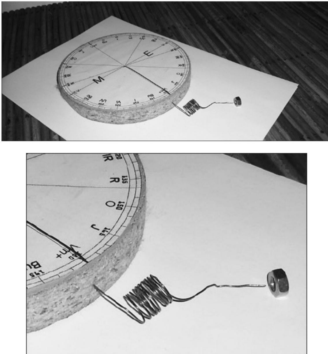
FIG. 14 : THE EXPERIMENT PROVING THE TRUE NATURE OF SHAPE EMISSIONS
