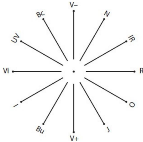
FIG. 4: THE SHAPE WAVES SPECTRUM
