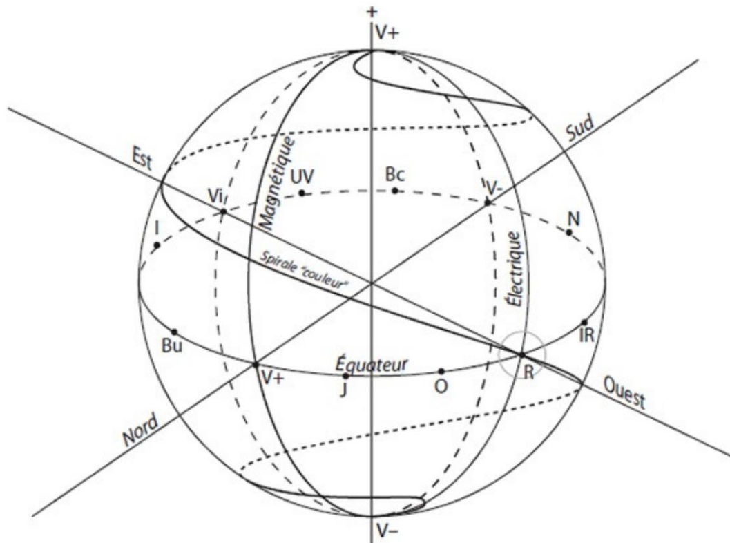
FIG. 3: THE SPHERE PROBED BY COLORED PENDULUMS
