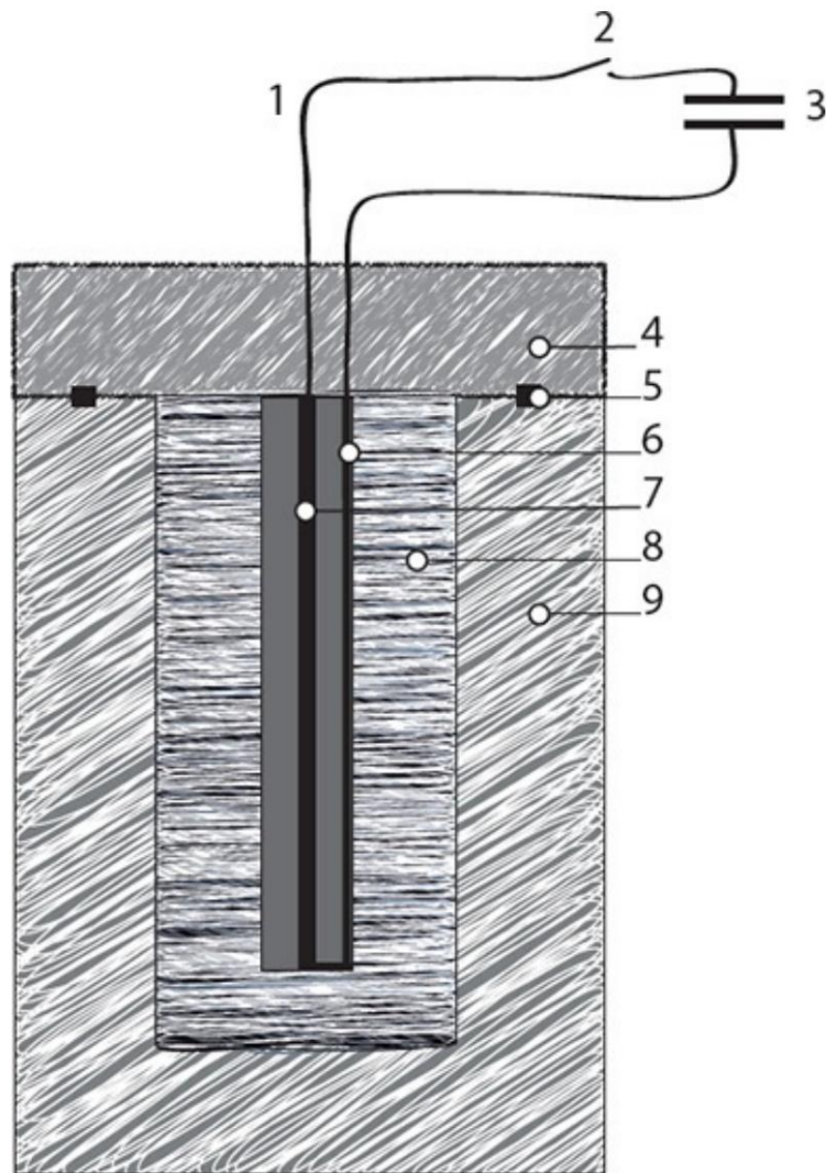
1. Cable – 2. Switch – 3. Capacitor bank 4. Plastic cover polyethylene – 5. Cover attachment 6. Foil – 7. Electrode – 8. Distilled water 9. Explosion chamber
