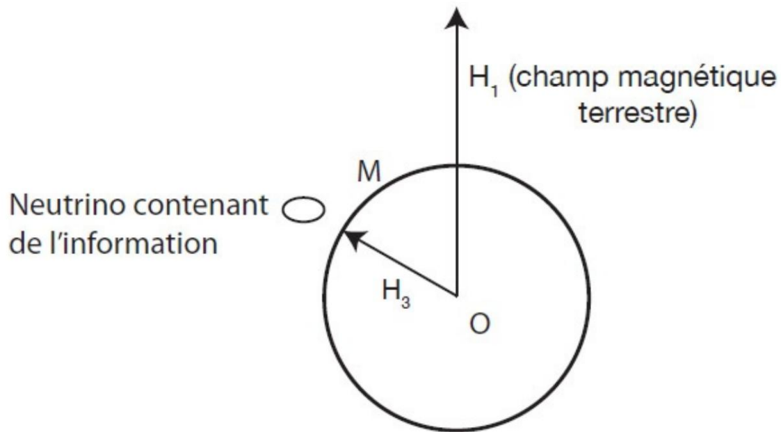
FIG. 8 : REPRESENTATION OF FIELDS H1 AND H3 FOR A SIMPLE FORM: THE CIRCLE
