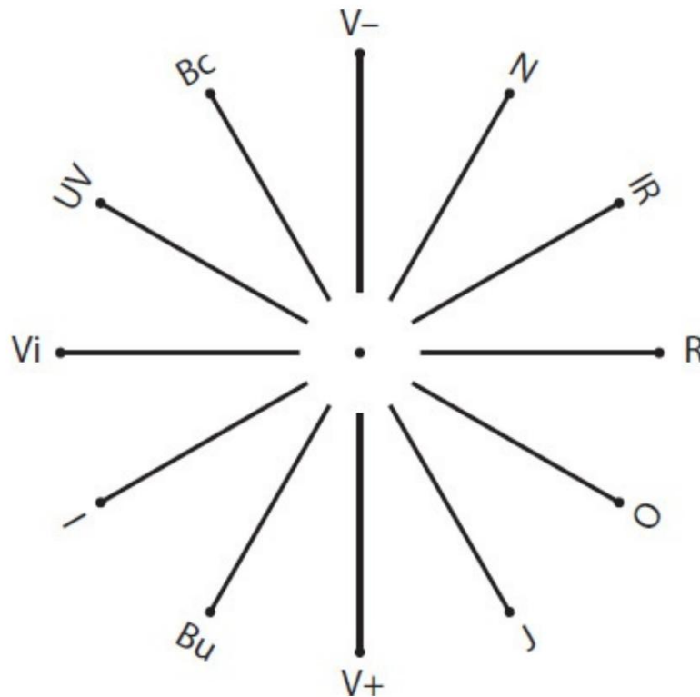
FIG. 1: THE SHAPE WAVES SPECTRUM
