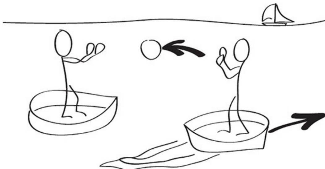
FIG. 17 : TWO BOATS INTERACT WITH THE EXCHANGE OF A BALLOON
