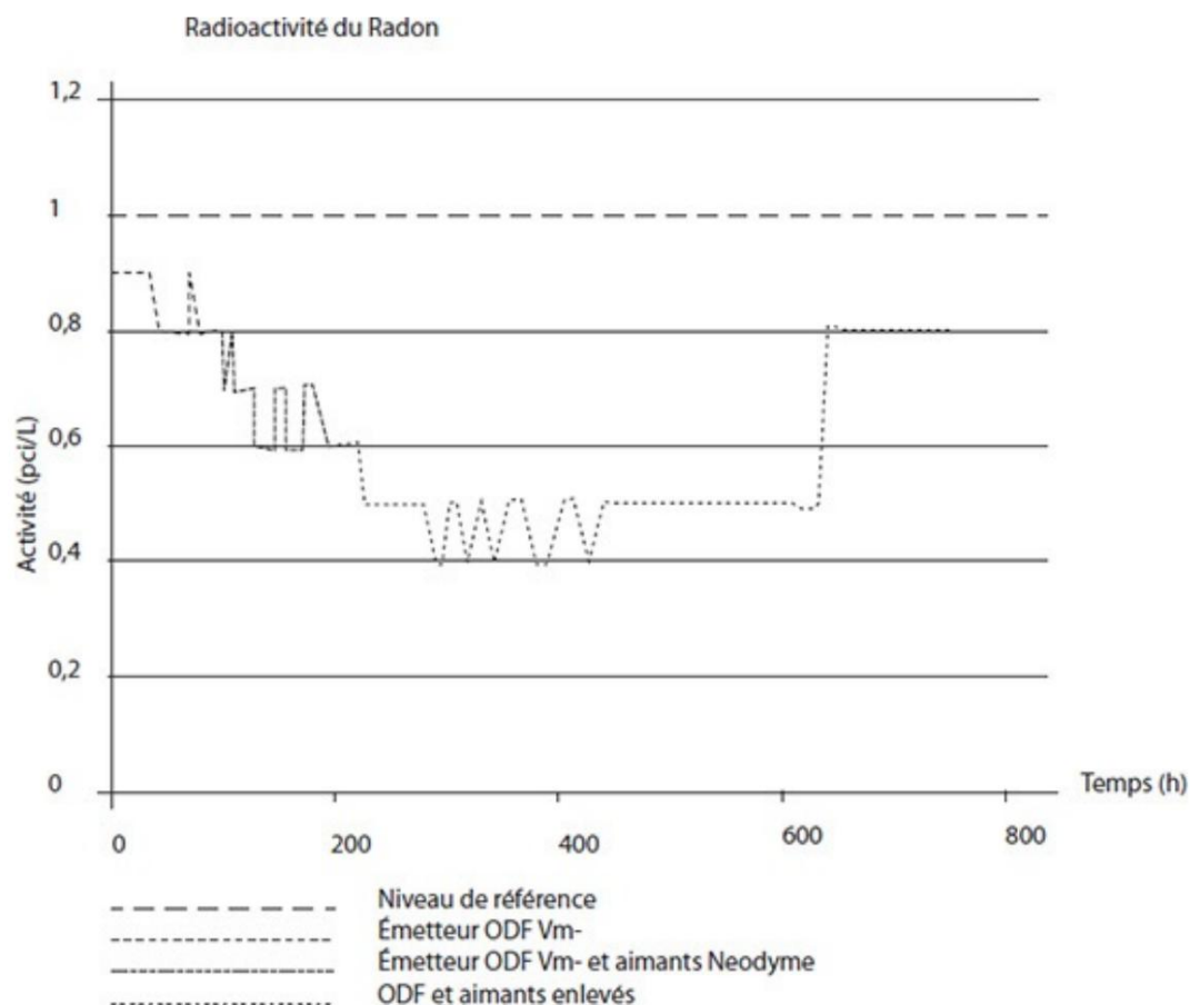
FIG. 19 : GRAPH SUMMARIZING ALL THE RADIOACTIVITY MEASUREMENTS OF RADON
