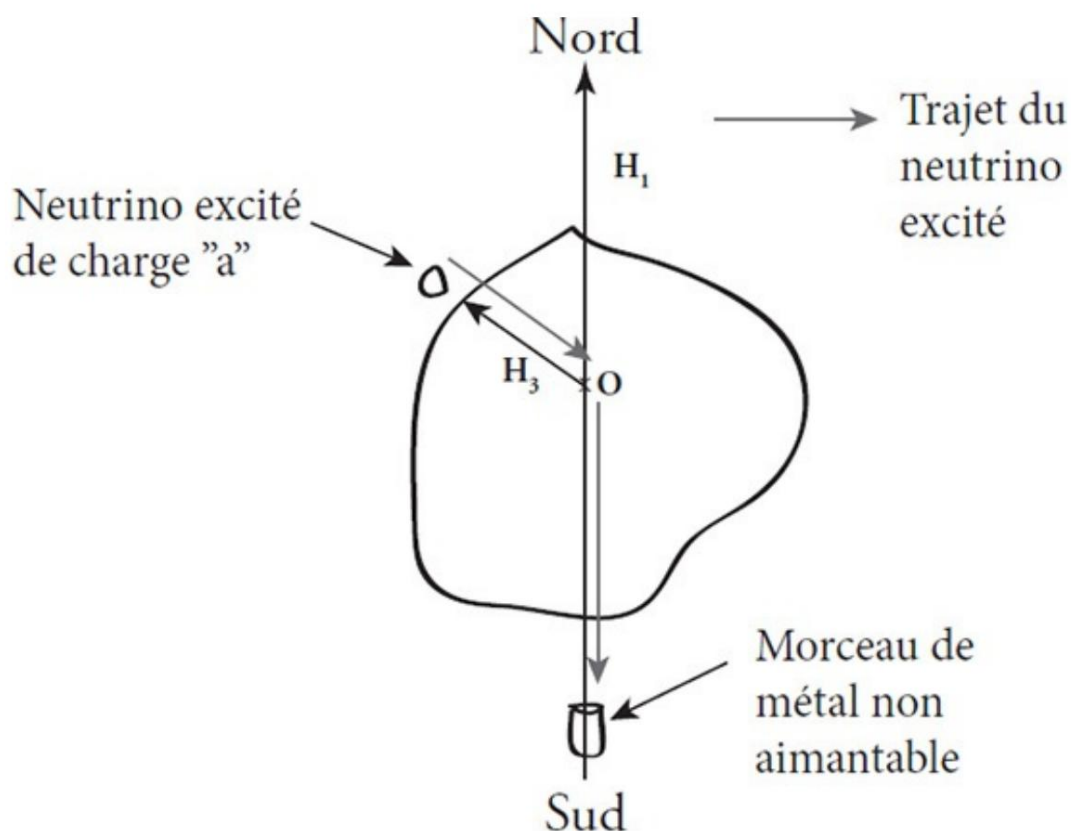
FIG. 16 : THE OPERATING PRINCIPLE OF THE EXPERIMENT IN FIGURE 14.
