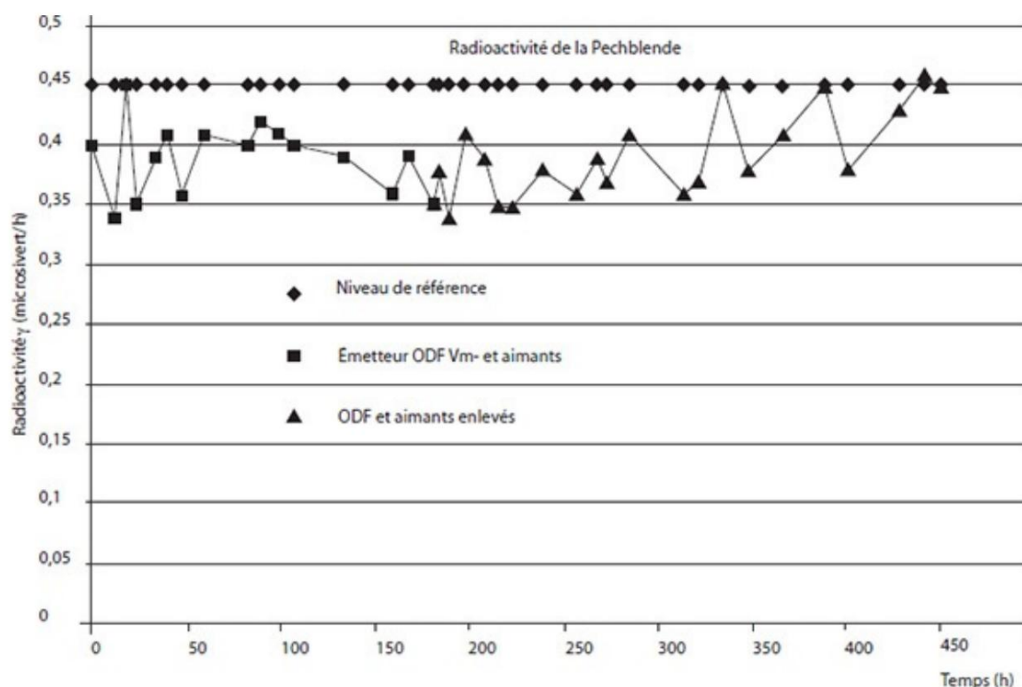
FIG. 21 : GRAPH SUMMARIZING PECHBLENDE RADIOACTIVITY MEASUREMENTS
