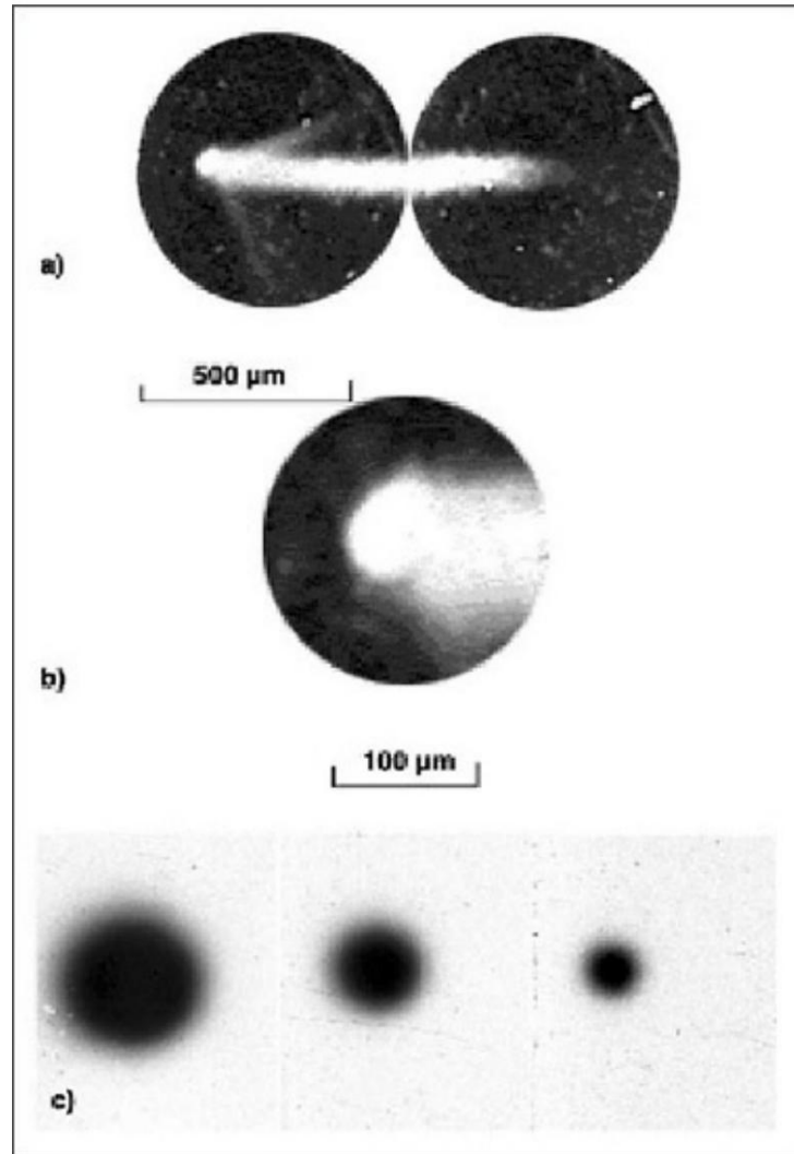
FIG. 12: THE STRANGE RADIATION PHOTOGRAPHED A) COMET-TYPE PLOT B) ENLARGEMENT OF THE COMET HEAD
